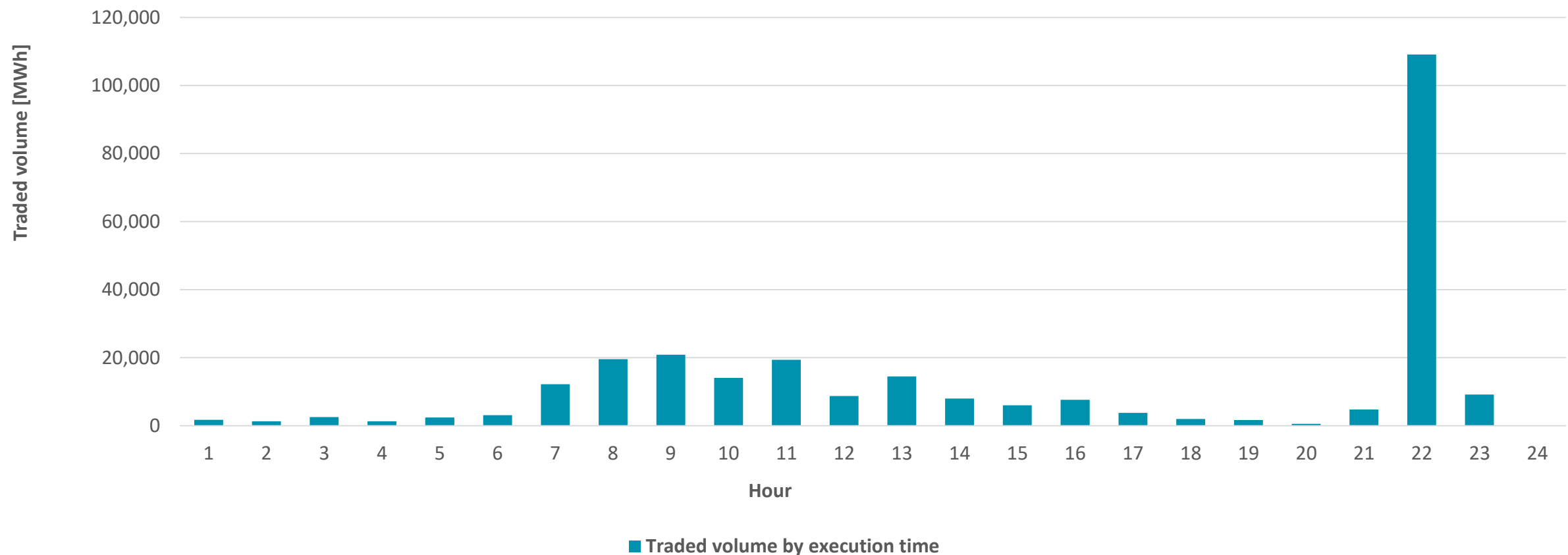
Traded volume during the day 19.11.2019-12.03.2020.
