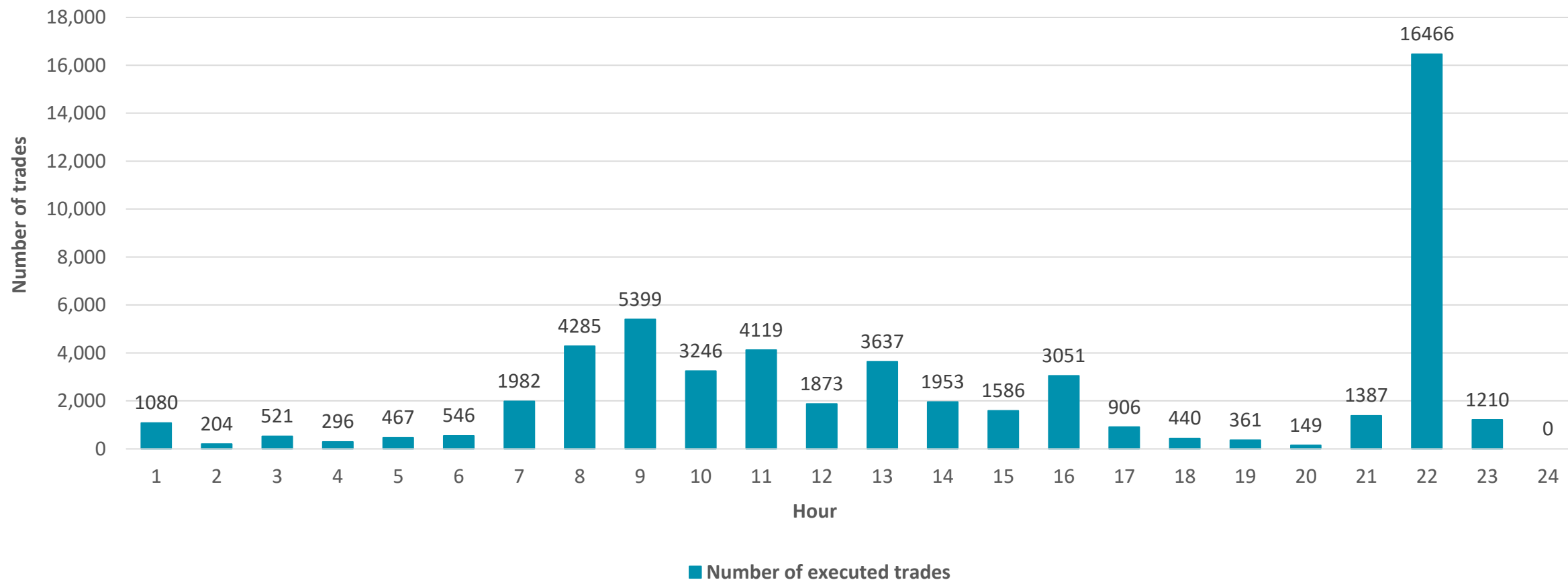
Number of trades during the day 19.11.2019-12.03.2020.
